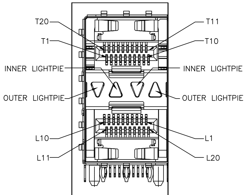
DETAIL A CIRCUIT NUMBERING AND LIGHTPIPE INDENTIRCATION
